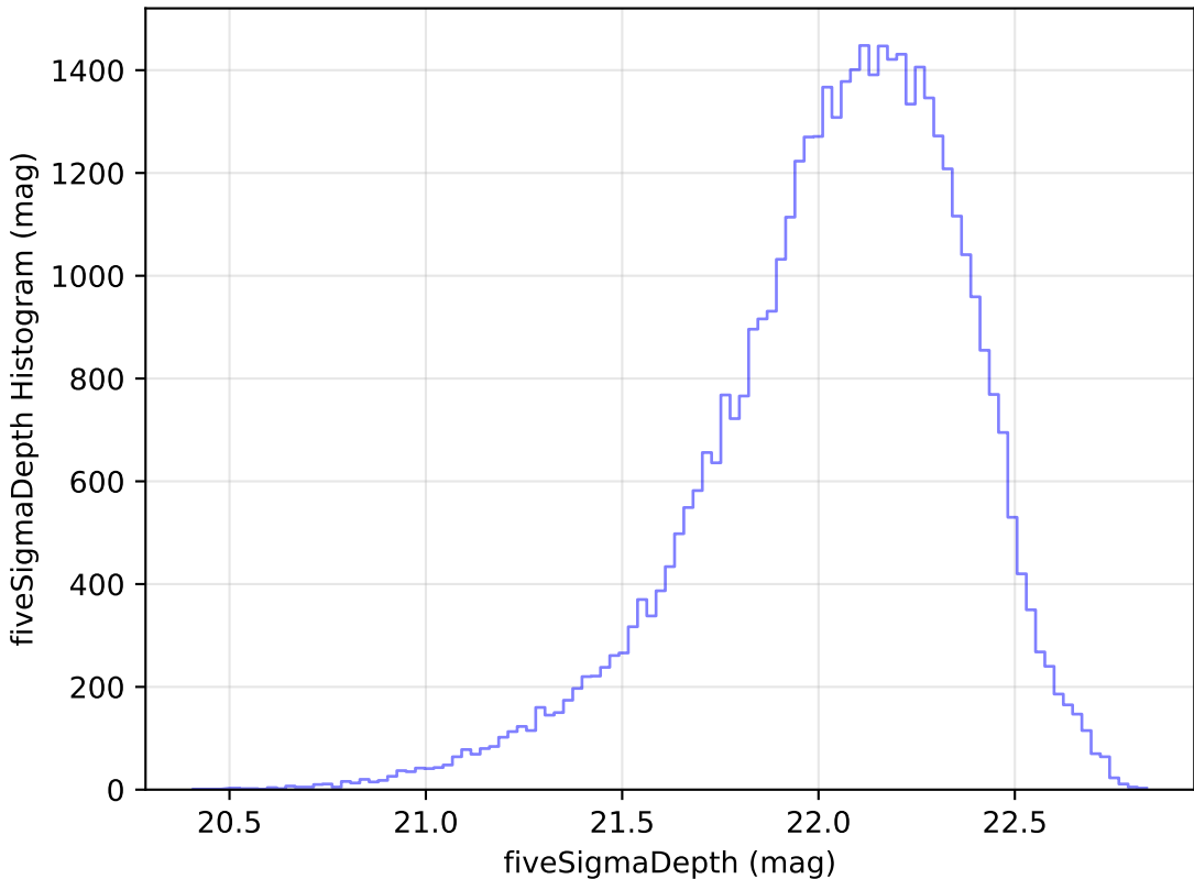
scp_reweight_v3.3_10yrs Yr 1 y band: fiveSigmaDepth Histogram
