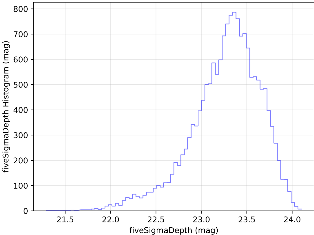
scp_reweight_v3.3_10yrs Yr 1 u band: fiveSigmaDepth Histogram
