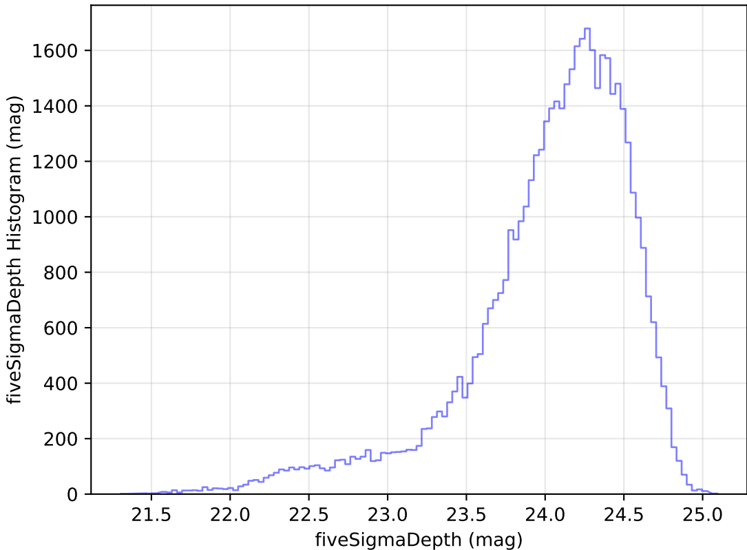
scp_reweight_v3.3_10yrs Yr 1 r band: fiveSigmaDepth Histogram
