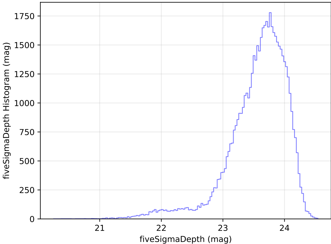
scp_reweight_v3.3_10yrs Yr 1 i band: fiveSigmaDepth Histogram
