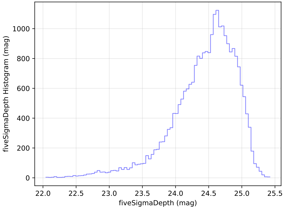
scp_reweight_v3.3_10yrs Yr 1 g band: fiveSigmaDepth Histogram
