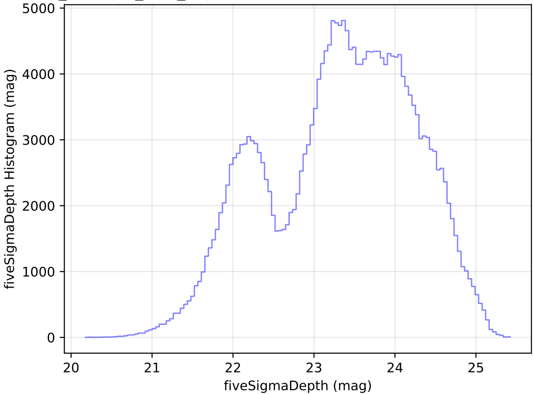
scp_reweight_v3.3_10yrs Yr 1 all bands: fiveSigmaDepth Histogram
