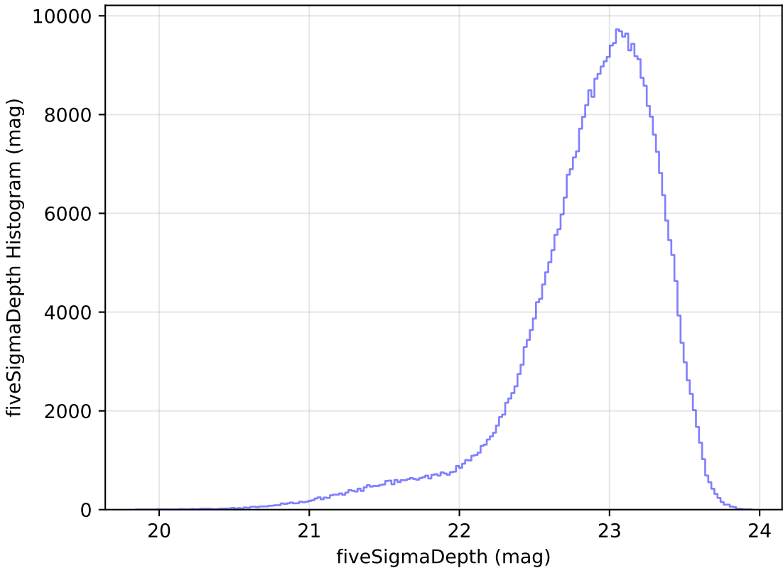
scp_reweight_v3.3_10yrs WFD z band: fiveSigmaDepth Histogram
