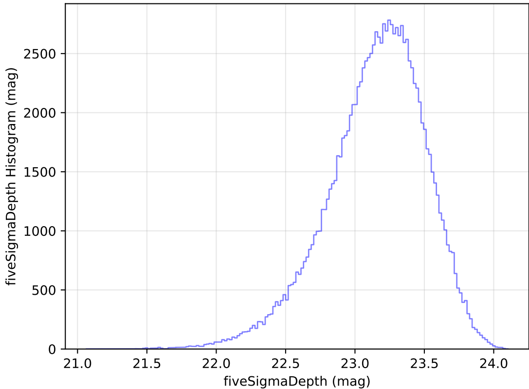
scp_reweight_v3.3_10yrs WFD u band: fiveSigmaDepth Histogram
