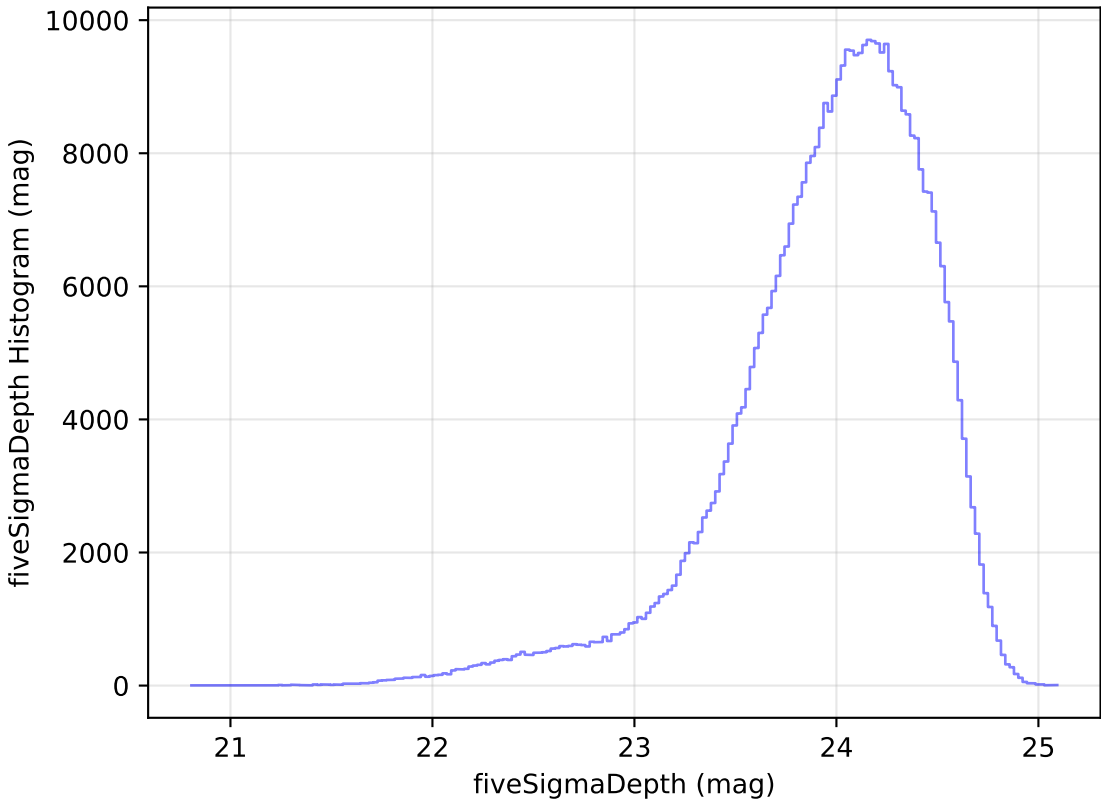
scp_reweight_v3.3_10yrs WFD r band: fiveSigmaDepth Histogram
