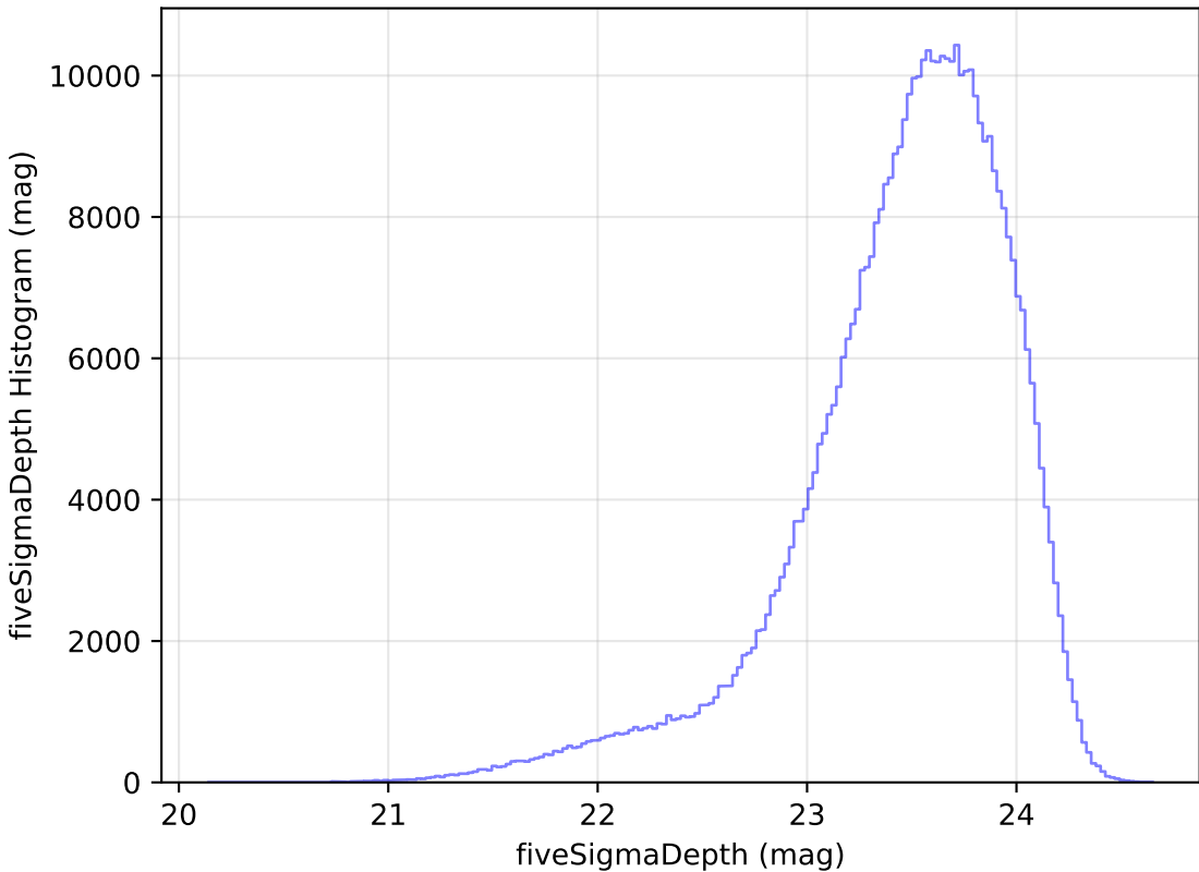
scp_reweight_v3.3_10yrs WFD i band: fiveSigmaDepth Histogram
