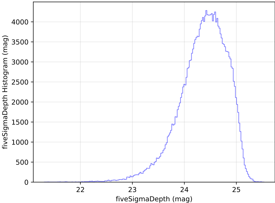
scp_reweight_v3.3_10yrs WFD g band: fiveSigmaDepth Histogram
