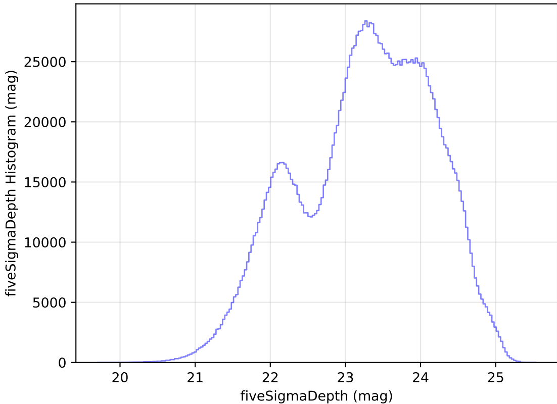
scp_reweight_v3.3_10yrs WFD all bands: fiveSigmaDepth Histogram
