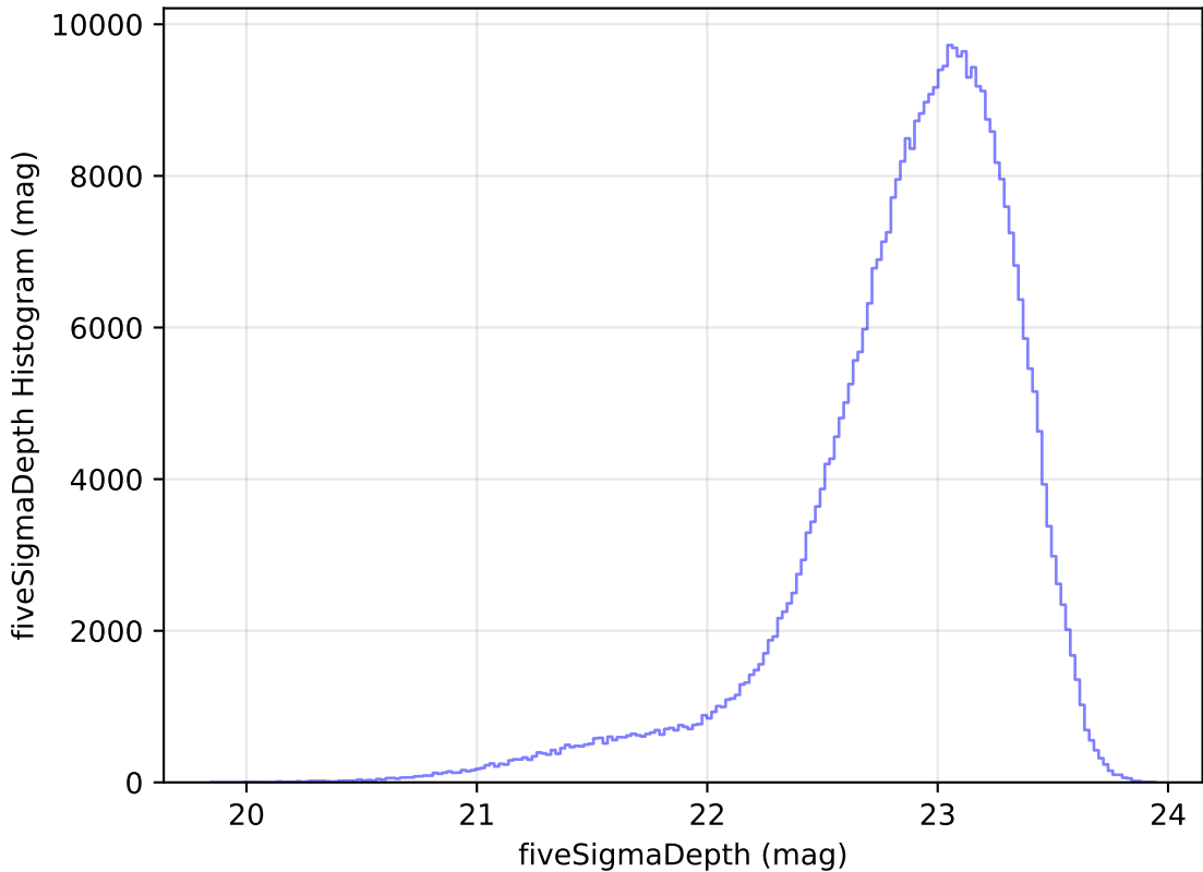
scp_reweight_v3.3_10yrs All sky z band: fiveSigmaDepth Histogram
