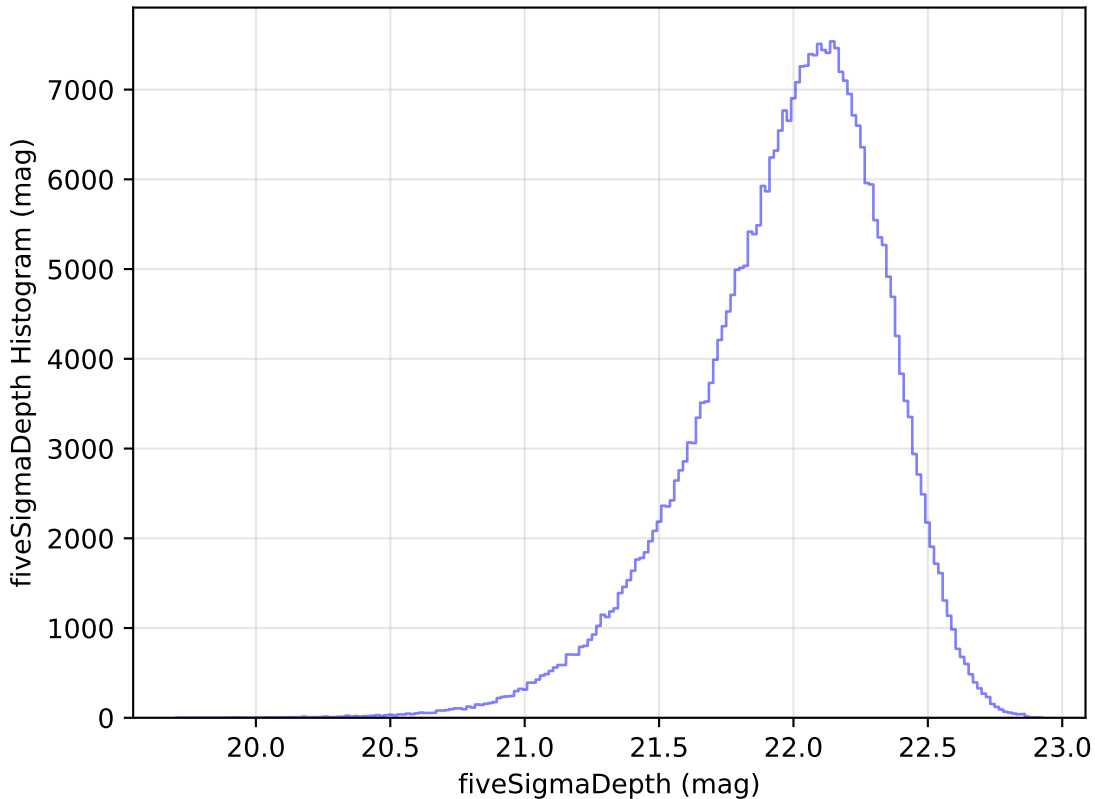
scp_reweight_v3.3_10yrs All sky y band: fiveSigmaDepth Histogram
