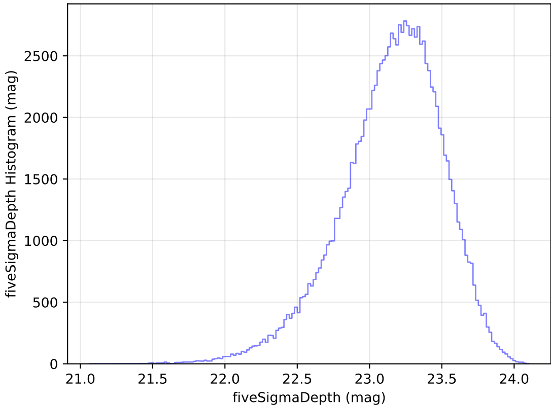
scp_reweight_v3.3_10yrs All sky u band: fiveSigmaDepth Histogram
