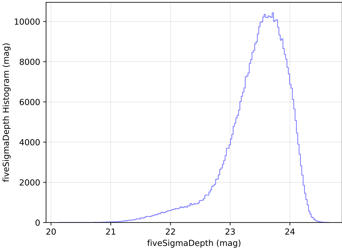
scp_reweight_v3.3_10yrs All sky i band: fiveSigmaDepth Histogram
