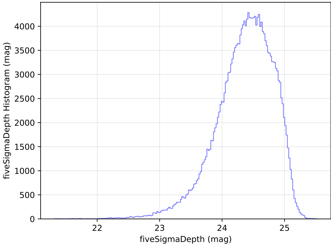
scp_reweight_v3.3_10yrs All sky g band: fiveSigmaDepth Histogram
