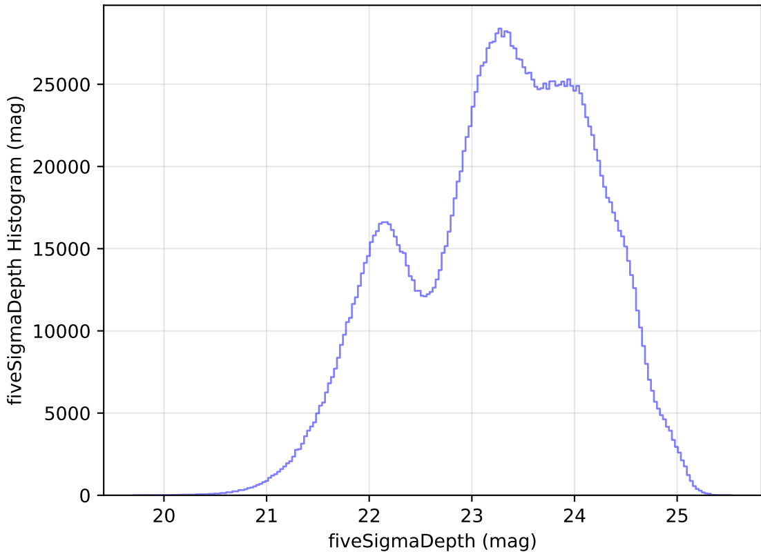
scp_reweight_v3.3_10yrs All sky all bands: fiveSigmaDepth Histogram
