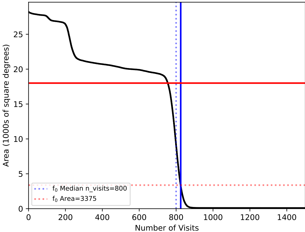
scp_reweight_v3.3_10yrs All sky: f0
