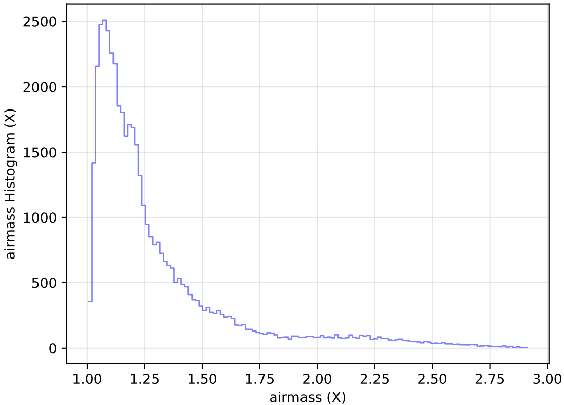
scp_reweight_v3.3_10yrs Yr 1 z band: airmass Histogram
