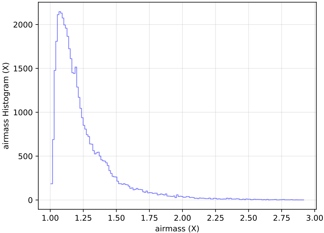
scp_reweight_v3.3_10yrs Yr 1 y band: airmass Histogram
