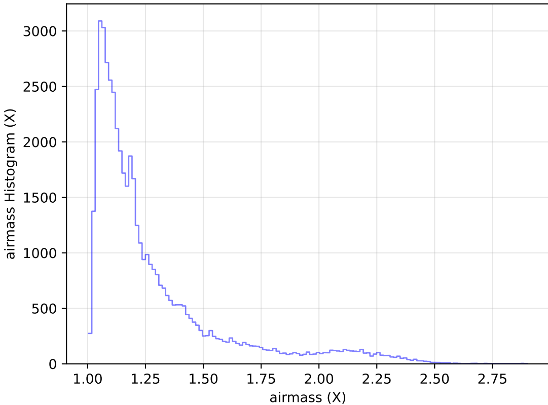
scp_reweight_v3.3_10yrs Yr 1 r band: airmass Histogram
