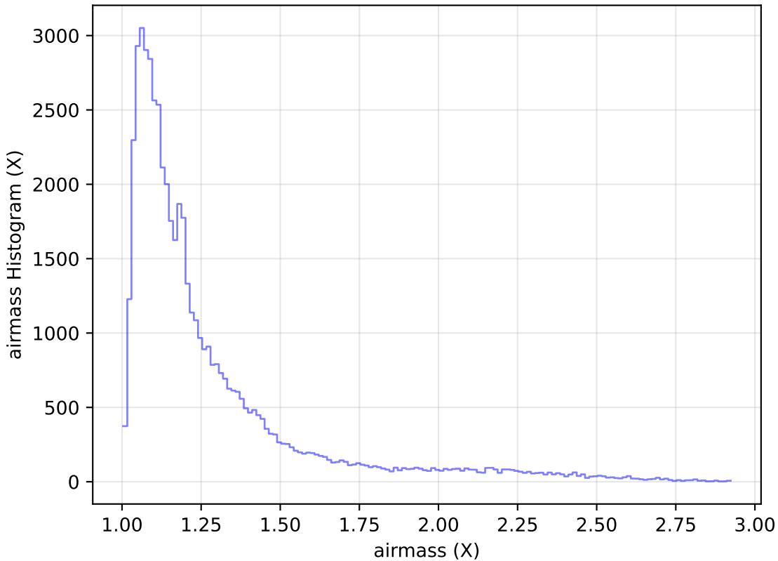
scp_reweight_v3.3_10yrs Yr 1 i band: airmass Histogram
