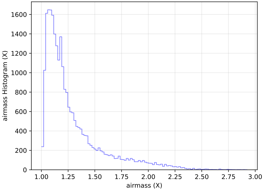
scp_reweight_v3.3_10yrs Yr 1 g band: airmass Histogram
