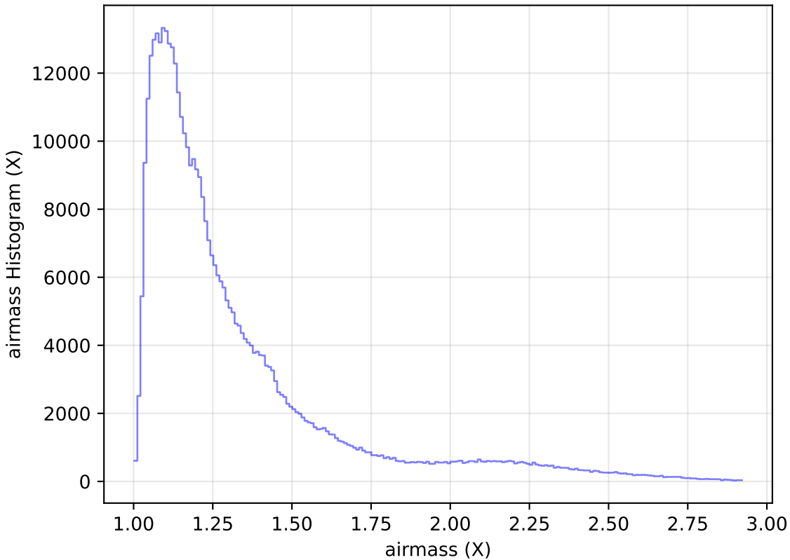
scp_reweight_v3.3_10yrs WFD z band: airmass Histogram
