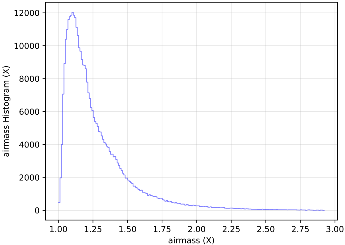
scp_reweight_v3.3_10yrs WFD y band: airmass Histogram
