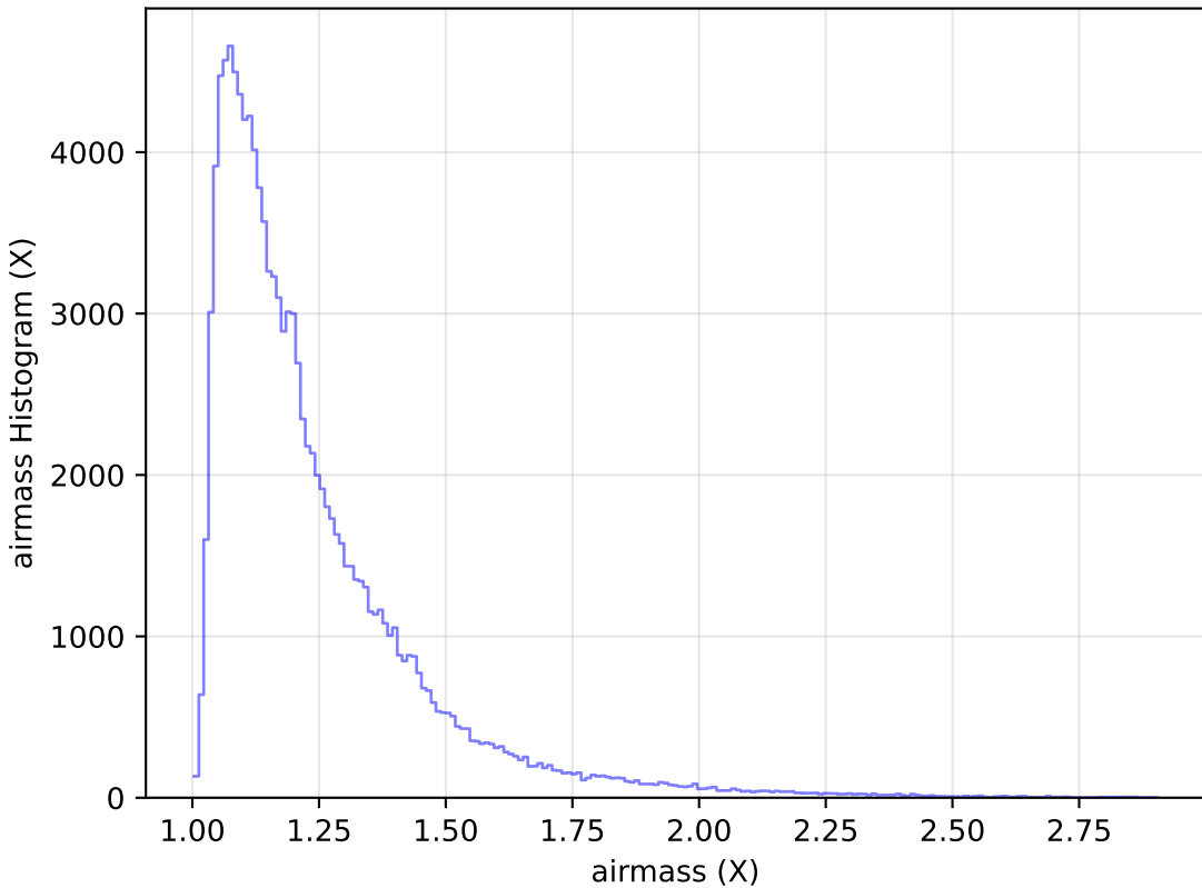
scp_reweight_v3.3_10yrs WFD u band: airmass Histogram
