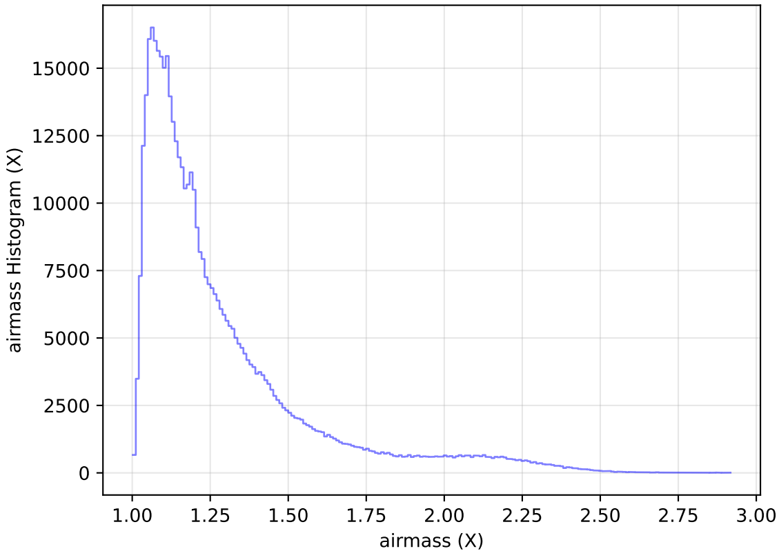
scp_reweight_v3.3_10yrs WFD r band: airmass Histogram
