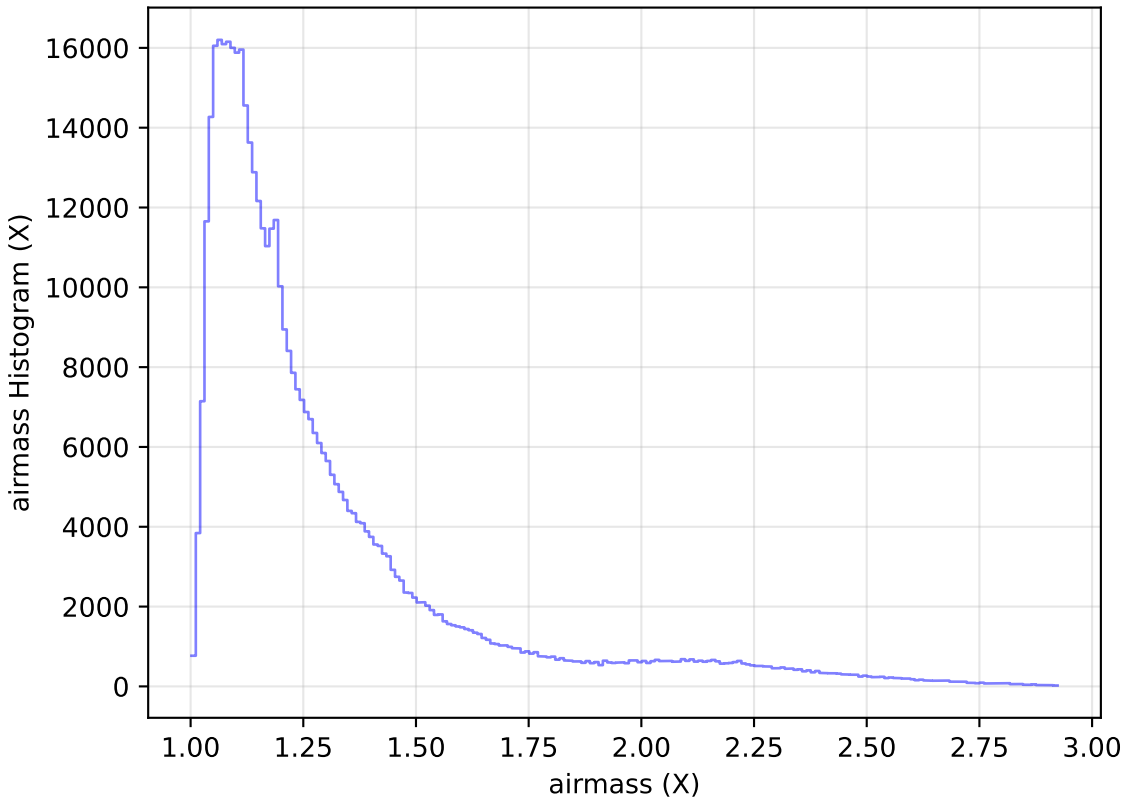
scp_reweight_v3.3_10yrs WFD i band: airmass Histogram
