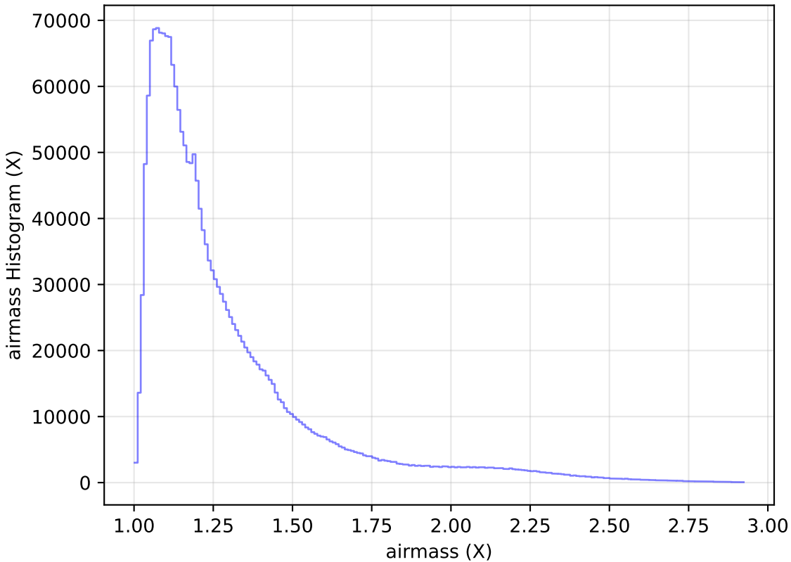
scp_reweight_v3.3_10yrs WFD all bands: airmass Histogram
