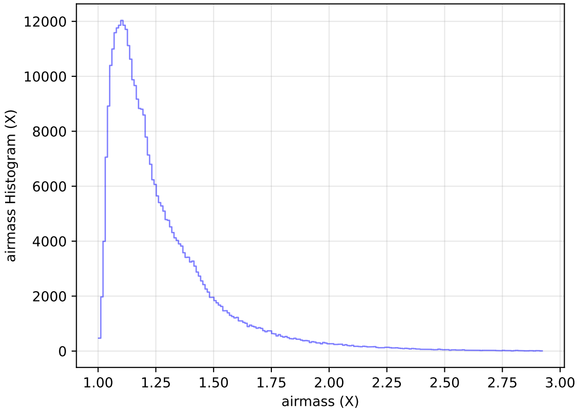
scp_reweight_v3.3_10yrs All sky y band: airmass Histogram
