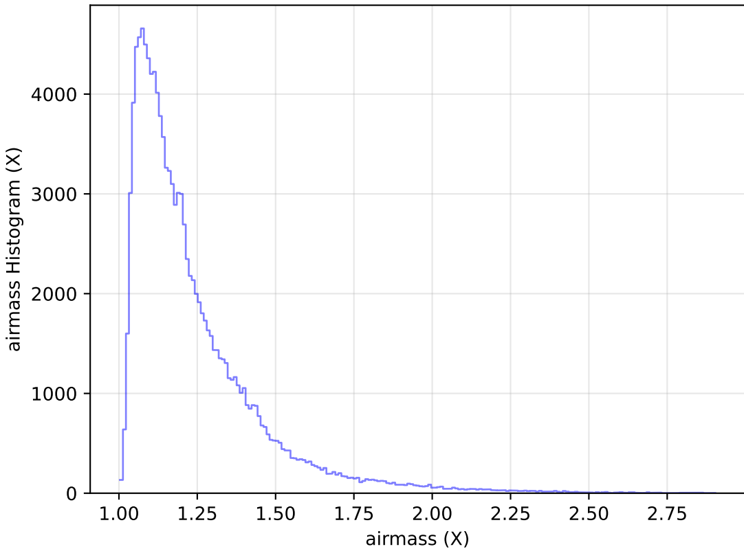
scp_reweight_v3.3_10yrs All sky u band: airmass Histogram
