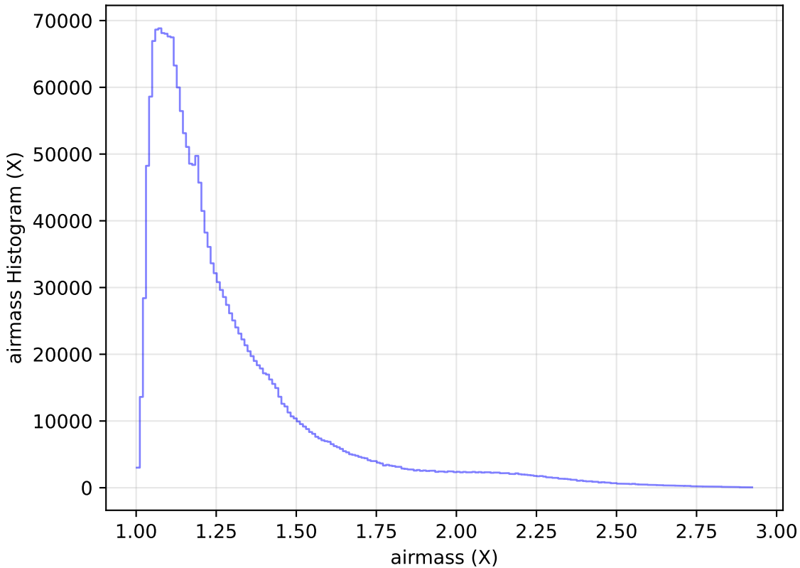
scp_reweight_v3.3_10yrs All sky all bands: airmass Histogram
