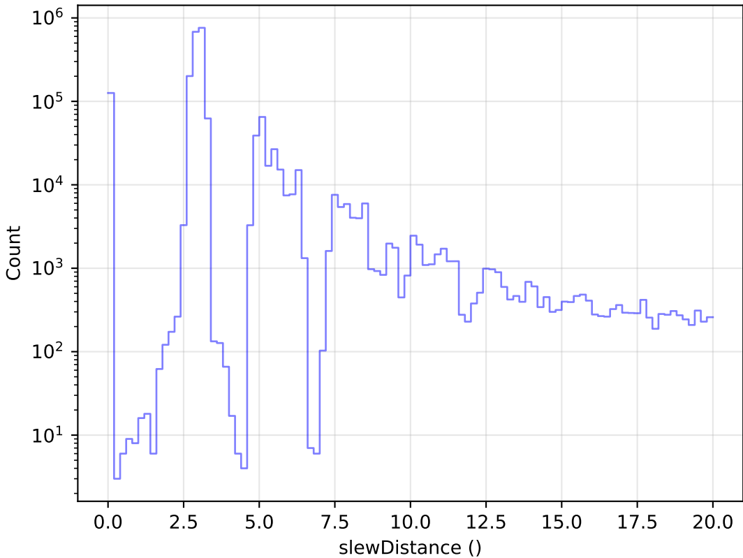
scp_reweight_v3.3_10yrs All visits: Zoom Slew Distance Histogram
