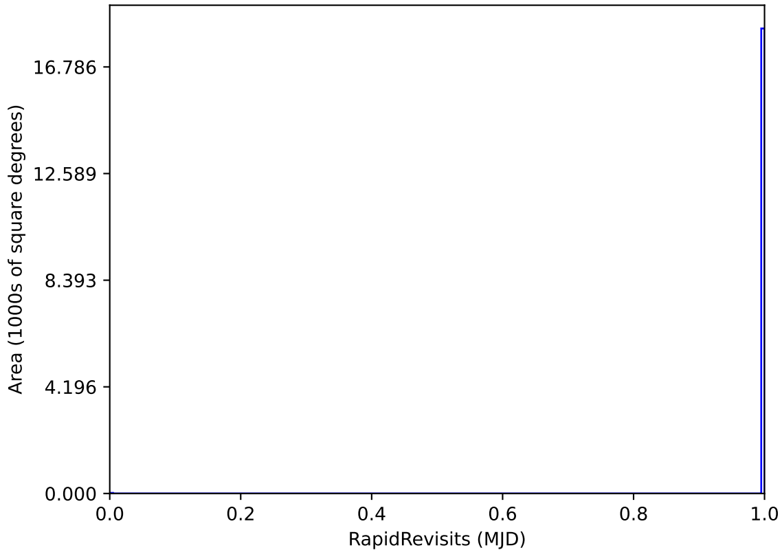
scp_reweight_v3.3_10yrs WFD: RapidRevisits
