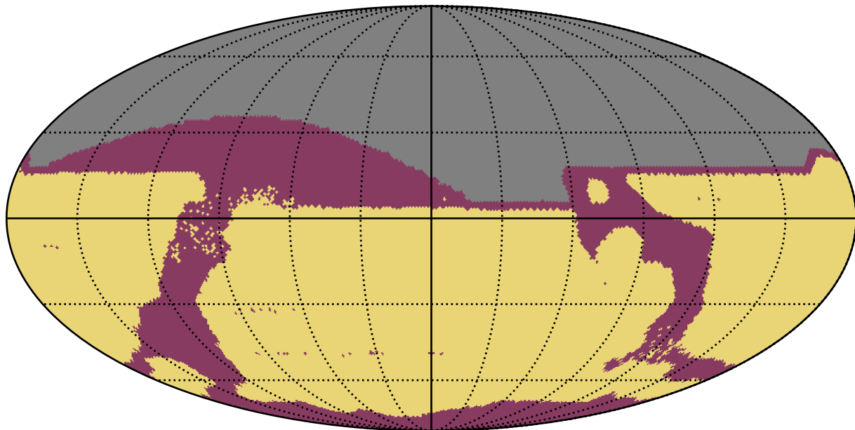
scp_reweight_v3.3_10yrs All sky: RapidRevisits
