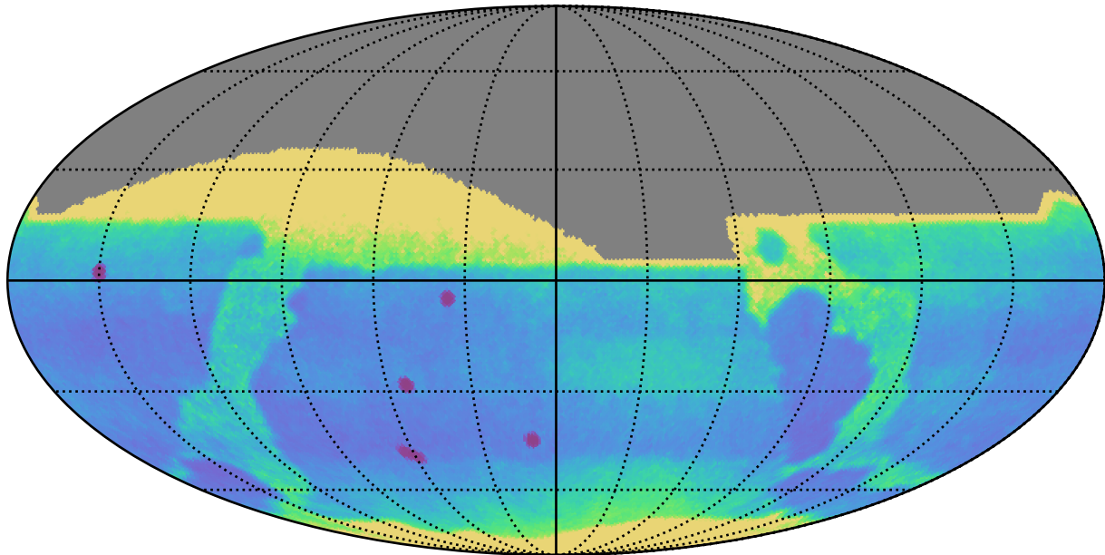
scp_reweight_v3.3_10yrs All sky: Proper Motion Uncert @ 24.0
