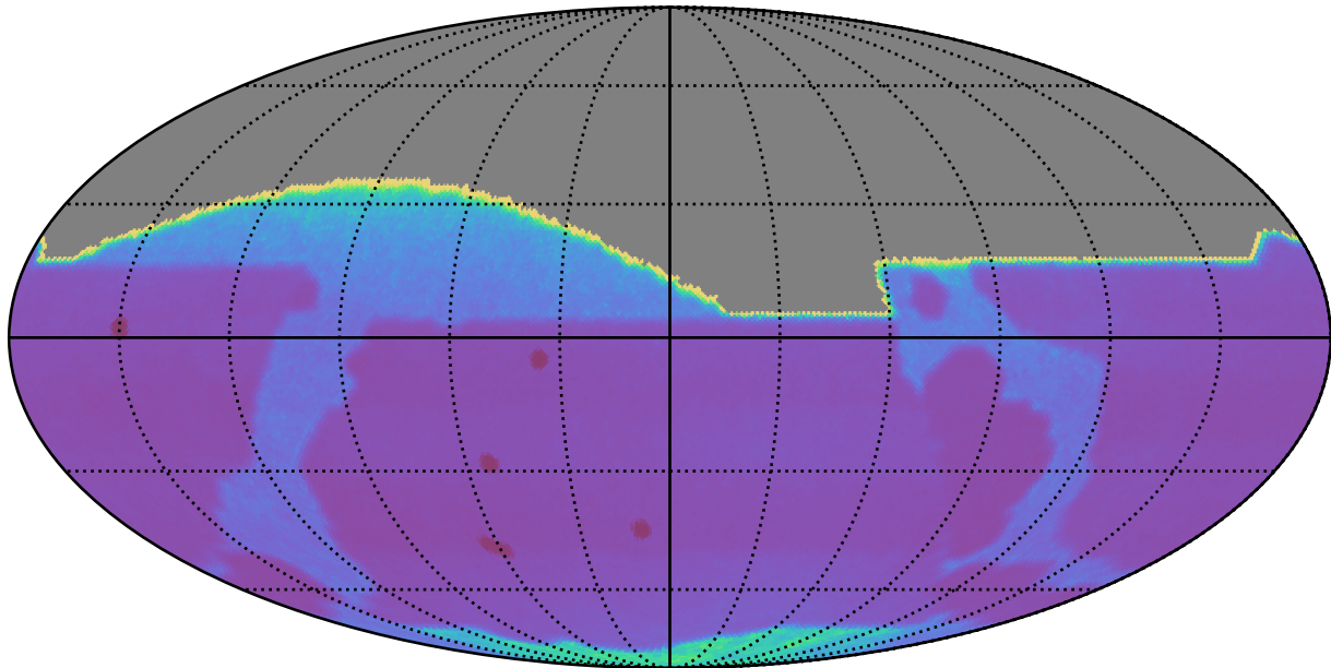
scp_reweight_v3.3_10yrs All sky: Proper Motion Uncert @ 20.5
