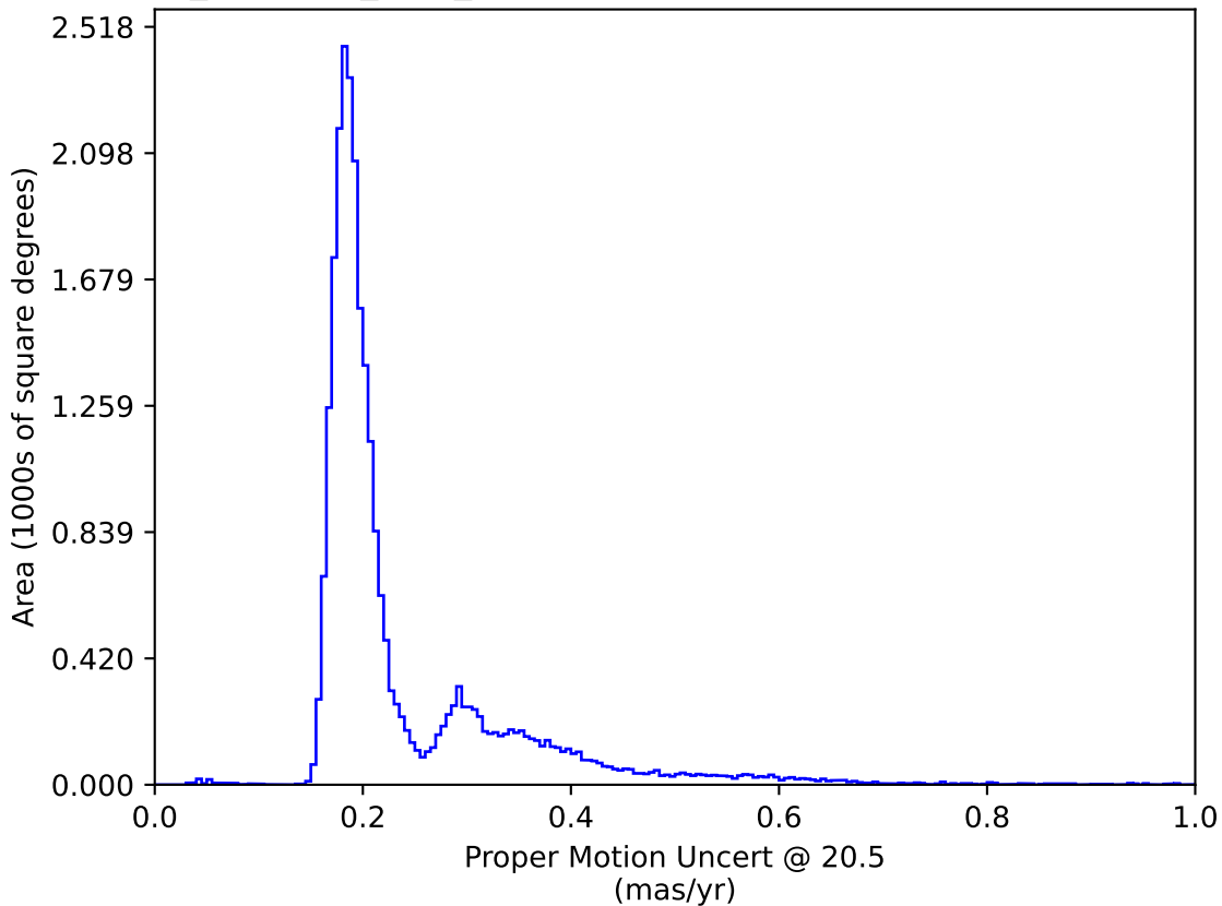
scp_reweight_v3.3_10yrs All sky: Proper Motion Uncert @ 20.5
