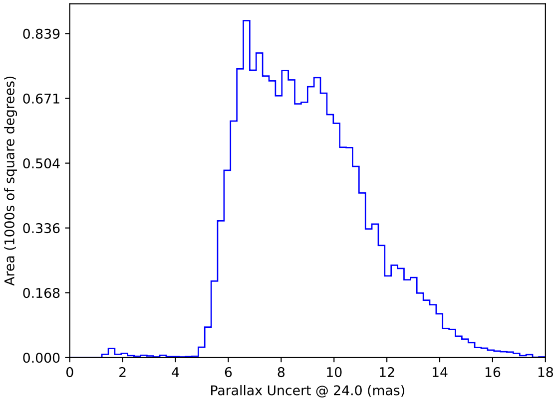
scp_reweight_v3.3_10yrs WFD: Parallax Uncert @ 24.0
