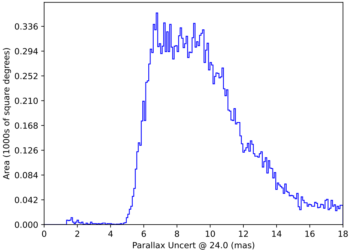
scp_reweight_v3.3_10yrs All sky: Parallax Uncert @ 24.0
