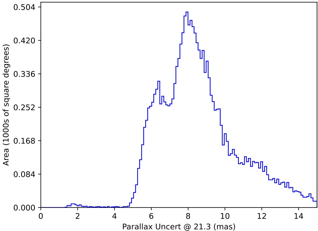
scp_reweight_v3.3_10yrs WFD y band only: Parallax Uncert @ 21.3
