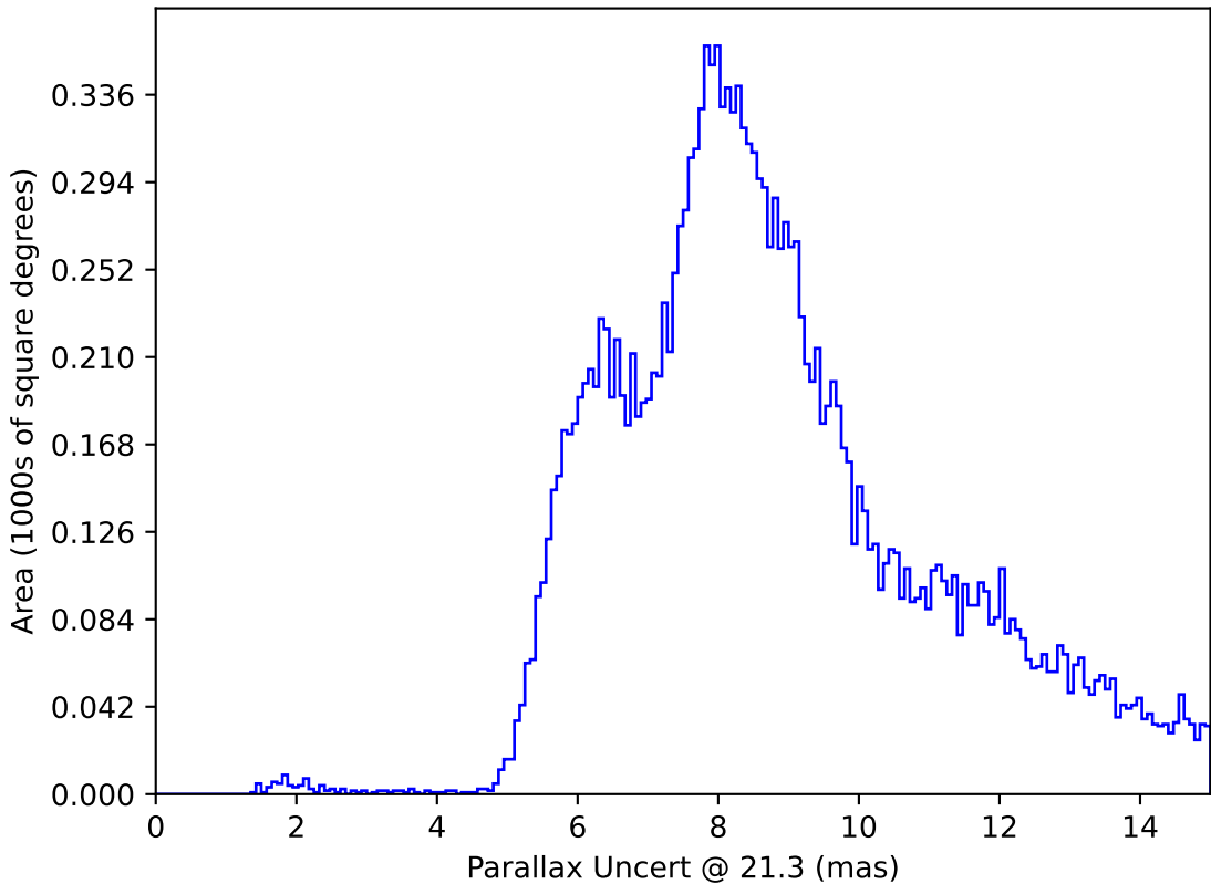
scp_reweight_v3.3_10yrs All sky y band only: Parallax Uncert @ 21.3
