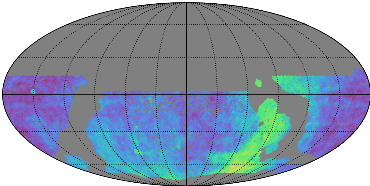
scp_reweight_v3.3_10yrs WFD: Parallax Coverage @ 24.0
