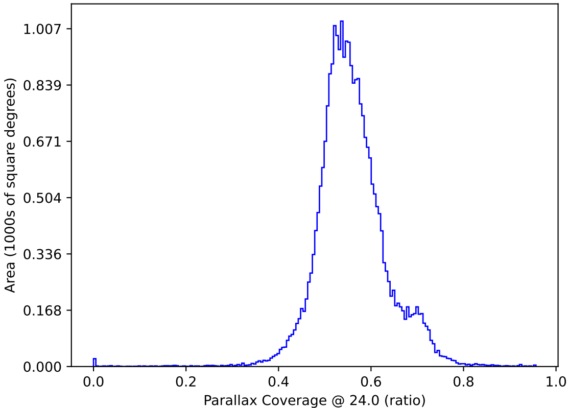
scp_reweight_v3.3_10yrs All sky: Parallax Coverage @ 24.0
