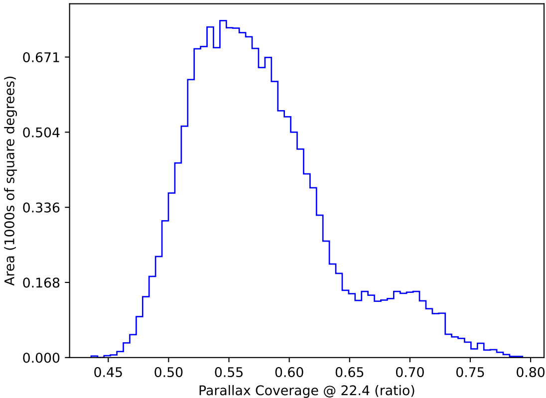
scp_reweight_v3.3_10yrs WFD: Parallax Coverage @ 22.4
