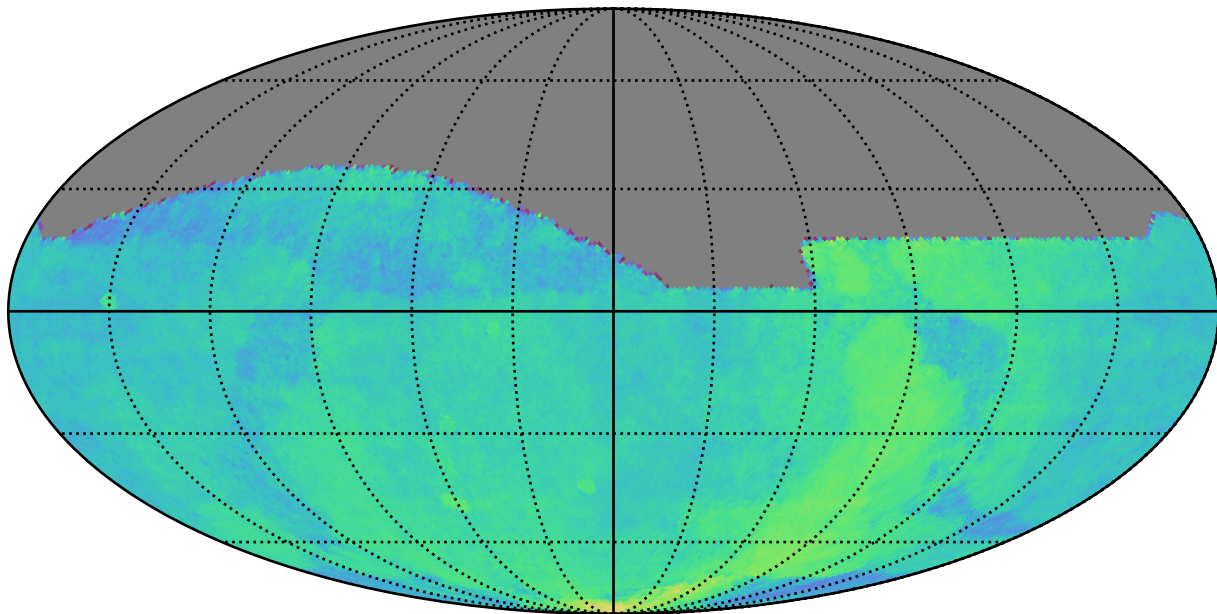
scp_reweight_v3.3_10yrs All sky: Parallax Coverage @ 22.4
