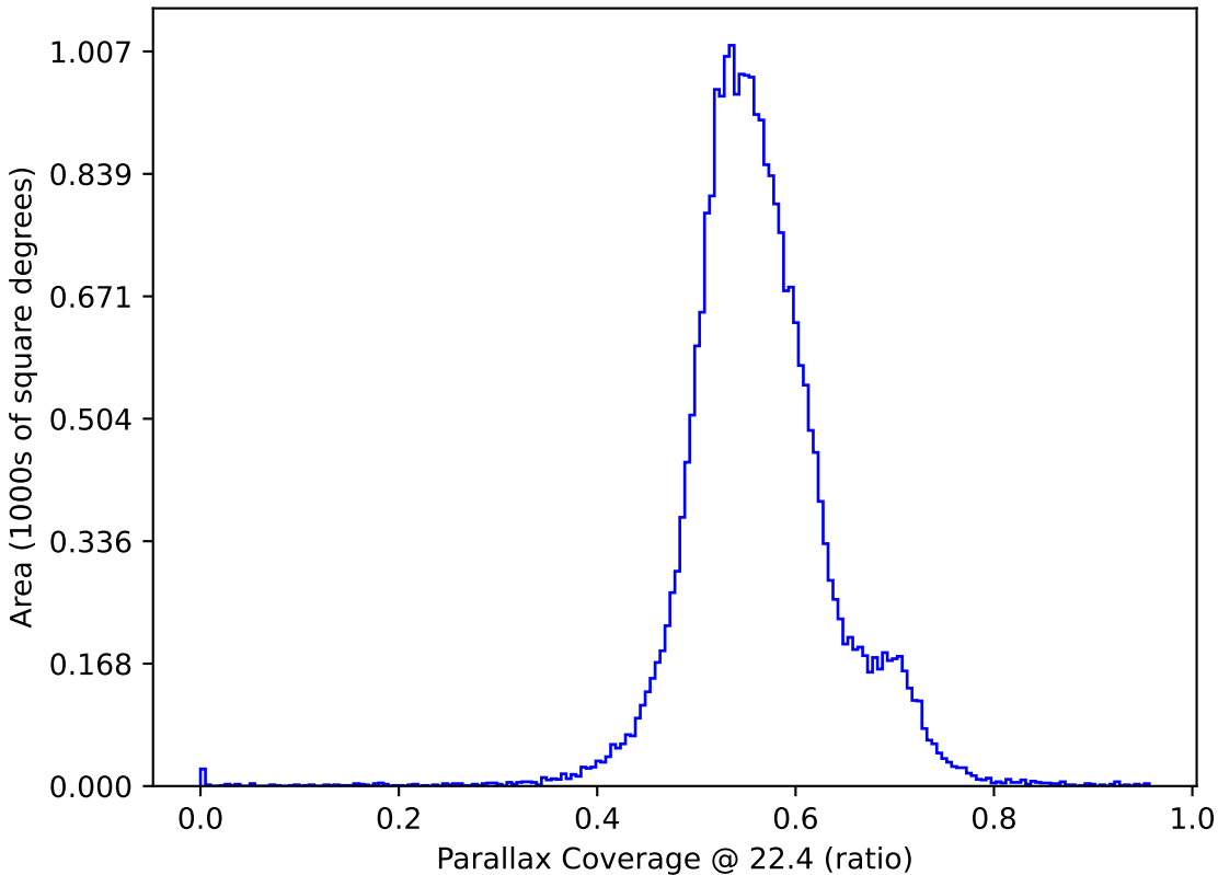
scp_reweight_v3.3_10yrs All sky: Parallax Coverage @ 22.4
