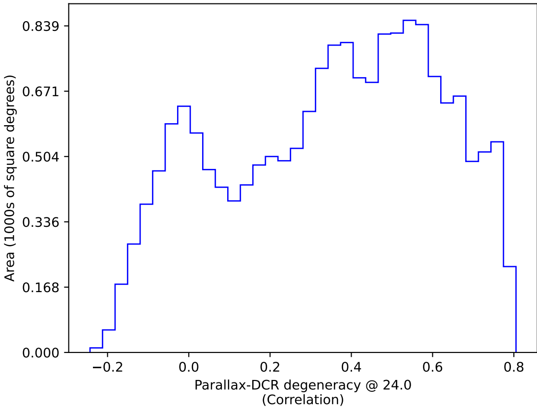
scp_reweight_v3.3_10yrs WFD: Parallax-DCR degeneracy @ 24.0
