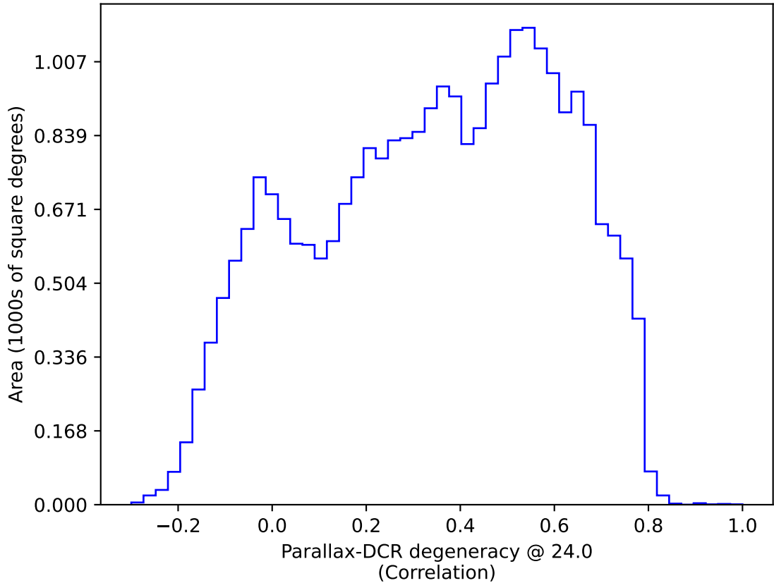
scp_reweight_v3.3_10yrs All sky: Parallax-DCR degeneracy @ 24.0
